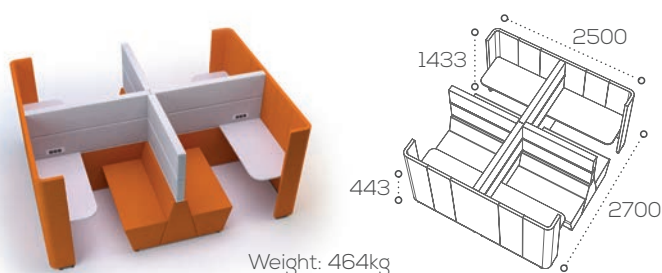
1200mm quad acoustic booth with bench SCE2B5
