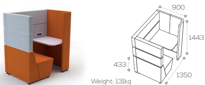
800mm single acoustic booth with bench SCE1B4
