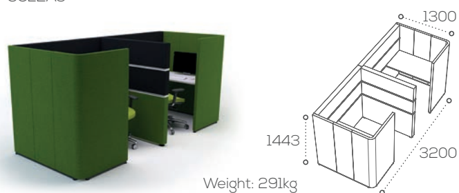
1200mm back-to-back double acoustic booth without bench SCE2A3
