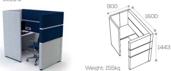
800mm single acoustic booth without bench SCE1A1
