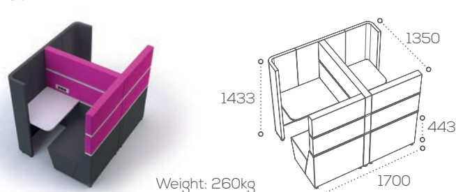
800mm side-by-side double acoustic booth with bench SCE1B2
