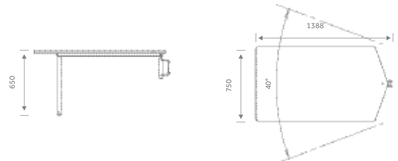
Dimensions (mm)
