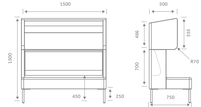
Dimensions (mm)
