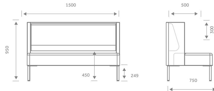
Dimensions (mm)
